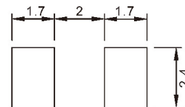
Top View Suggested Layout
